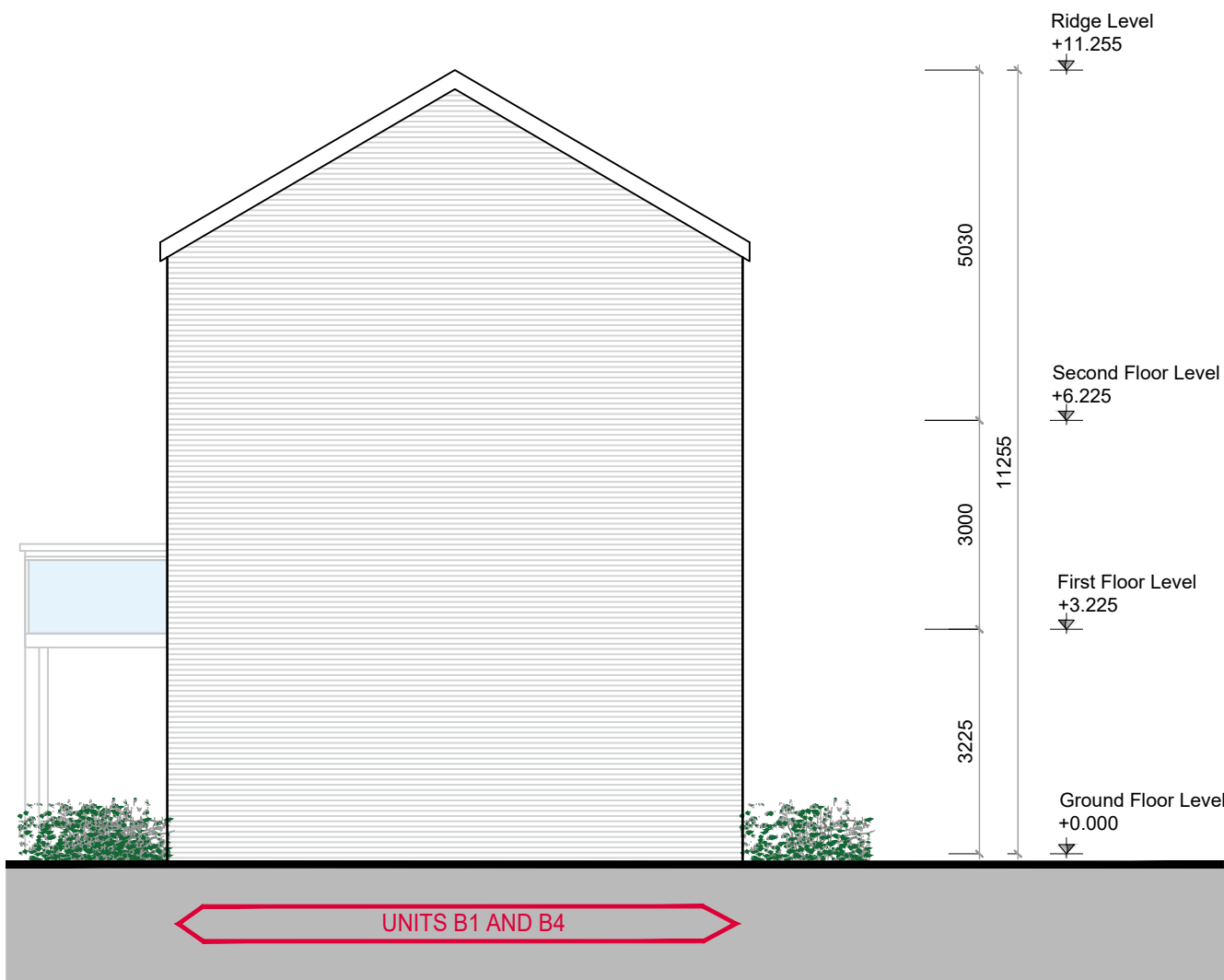
EAST ELEVATION
